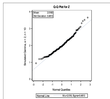
Figure 11. Gamma, \alpha = 2, n = 10
