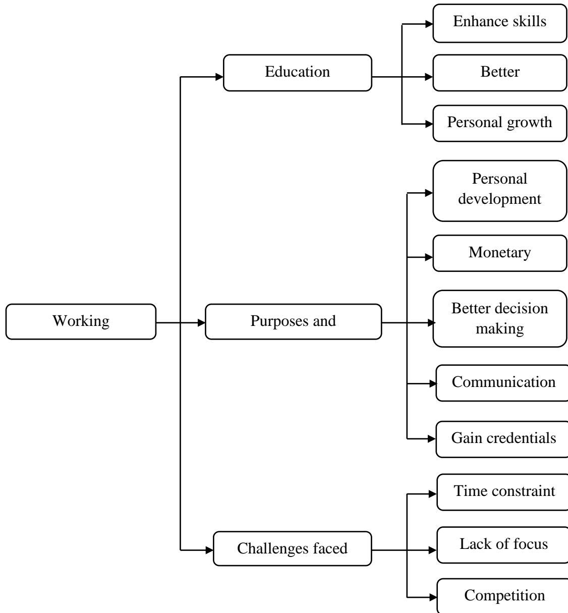
Figure 1: Coding hierarchy
