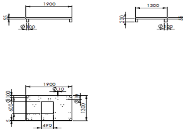
Figure 5: Dimensions of the platform
