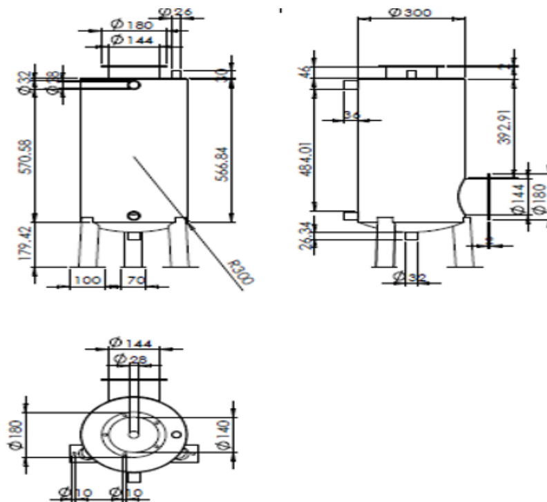
Figure 9: Dimensions of carbon and sediment units
