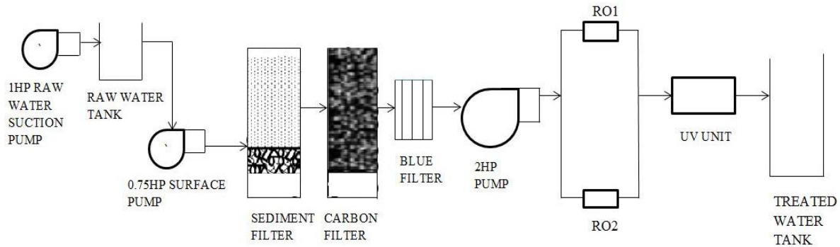
Figure 3: Schematic representation of the treatment flow process for the mobile treatment unit.
