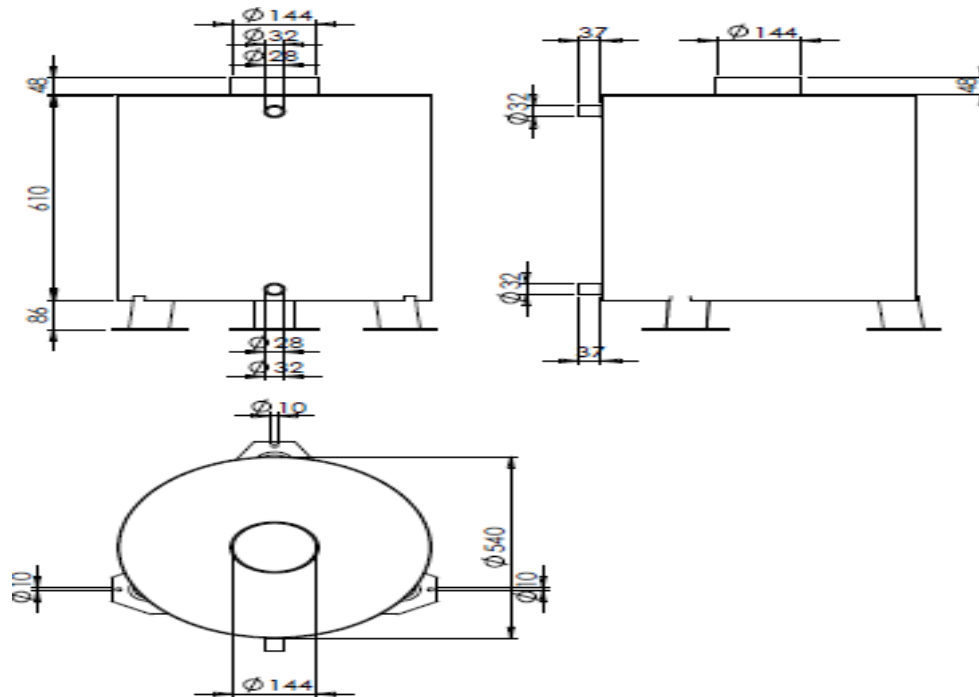
Figure 7: Dimensions of the raw and treated water tanks
