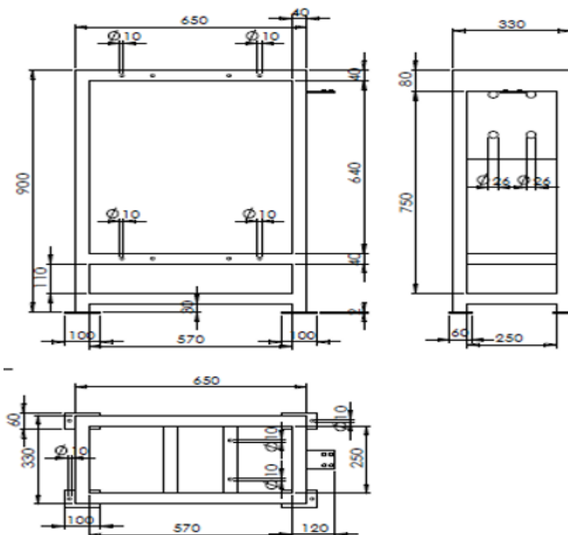
Figure 11: Dimensions of the Frame
