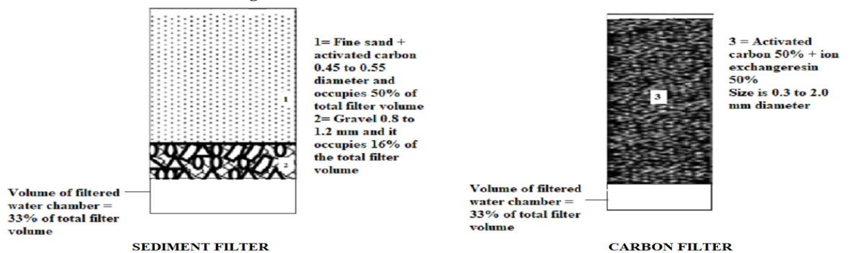
Figure 9: Dimensions of carbon and sediment units
