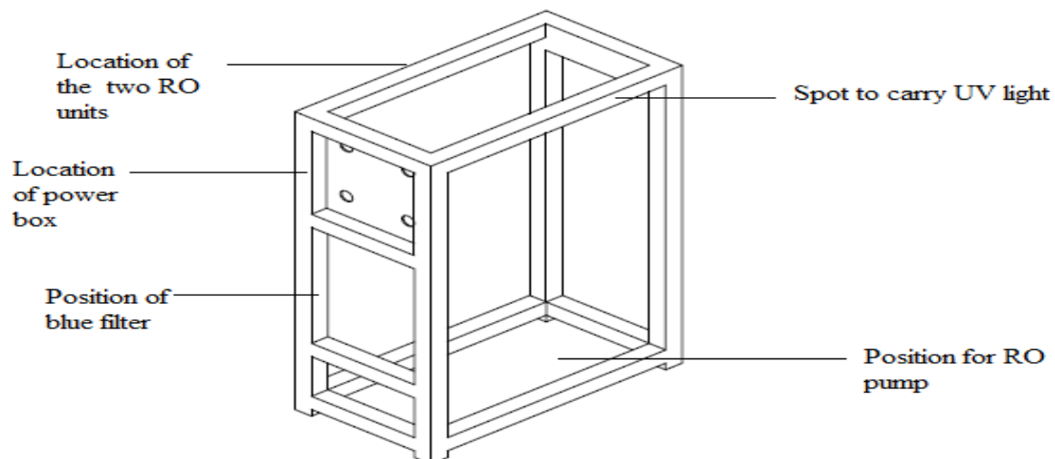
Figure 9: Frame
